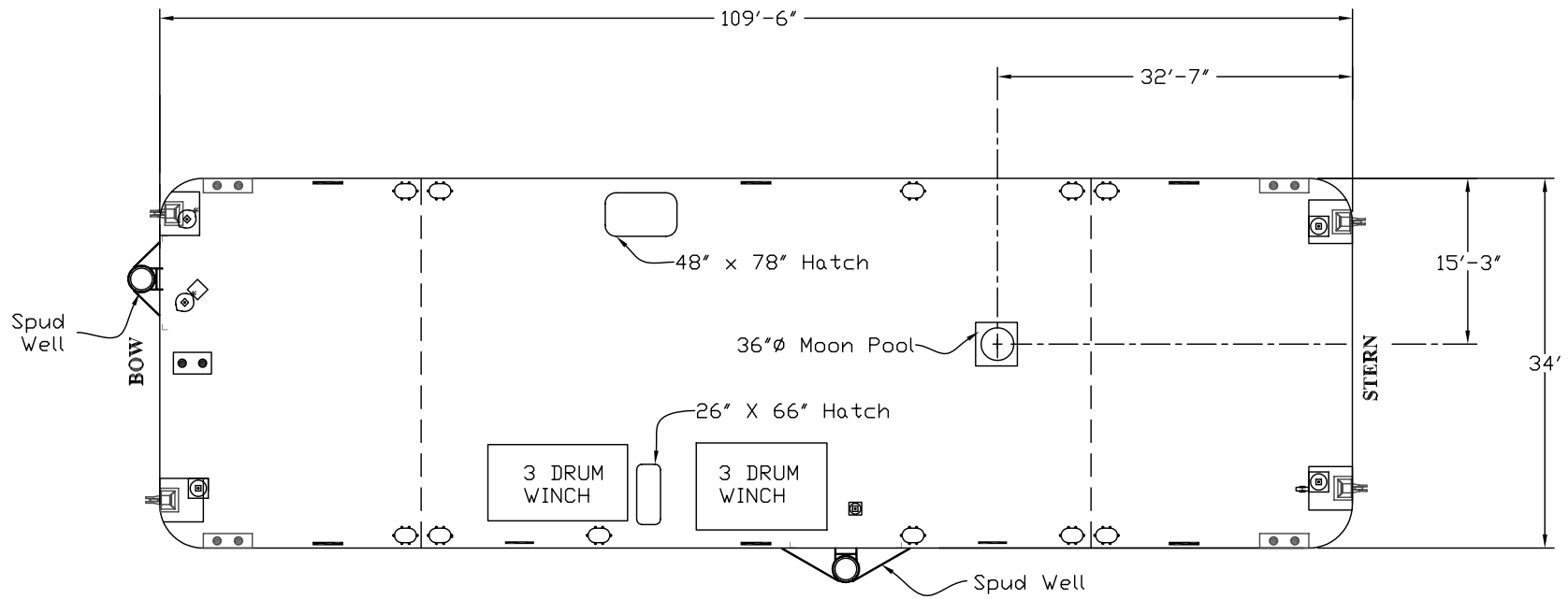
CSM 39 - Deck Plan
