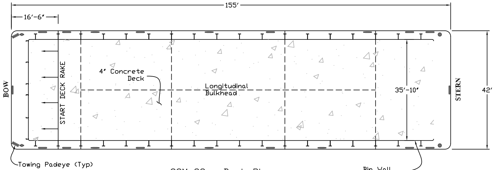
CSM 28 - Deck Plan
