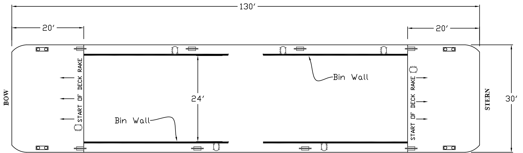
CSM 49 - Deck Plan
