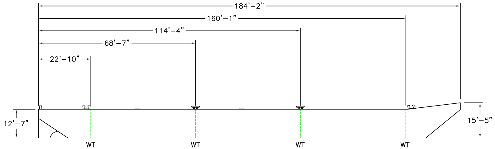
PROFILE - Barge 31
