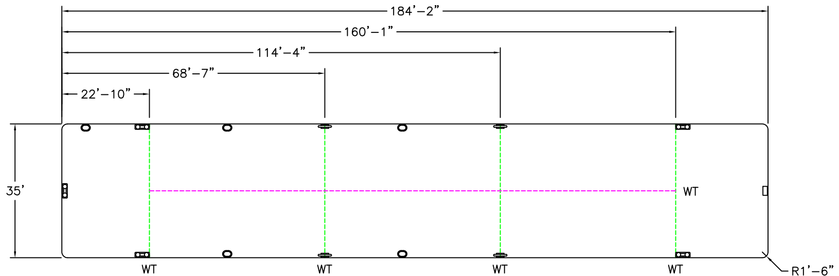
PLAN - Barge 31
