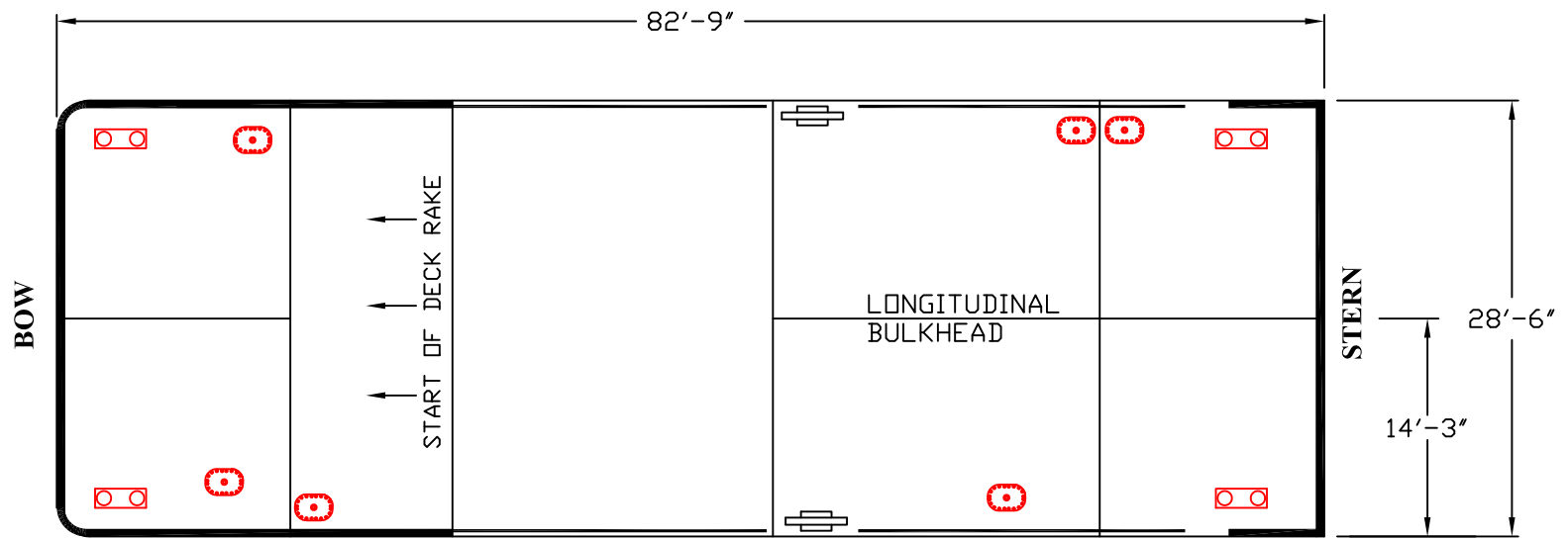
CSM 23 - Deck Plan
